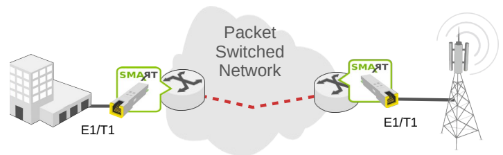
Plug-and play E1/T1 transport over Packet
